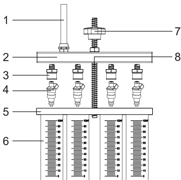
Top-in fuel injector installation diagram
